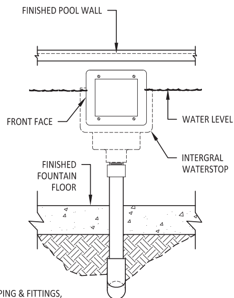
ELEVATION VIEW
